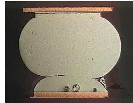
Pillow defect
